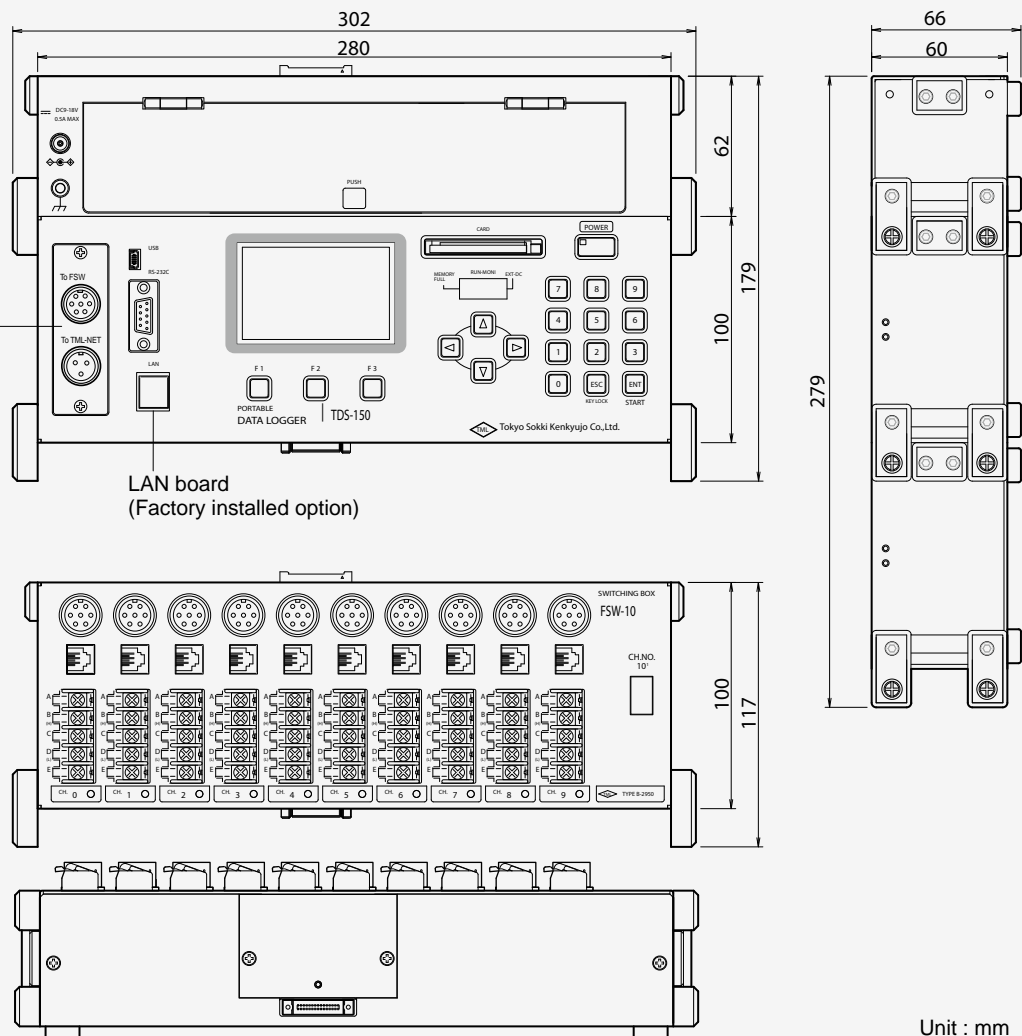
TDS-150 Control unit (Battery unit included)
