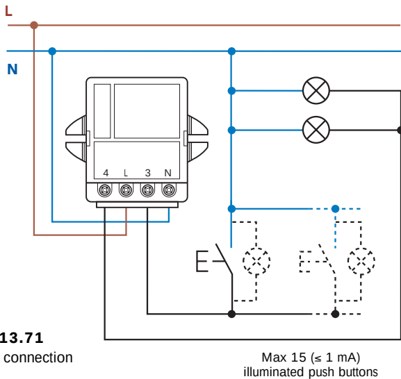
Type 13.71 4 wire connection
