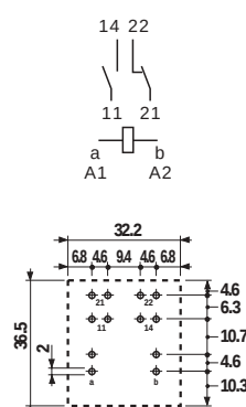
Copper side view
