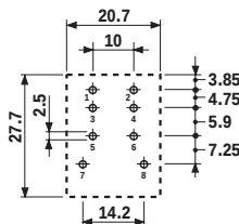
Copper side view h = 37.7 mm
