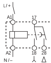
star - delta
