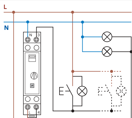
4 wire connection
