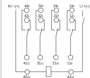
wiring diagram
