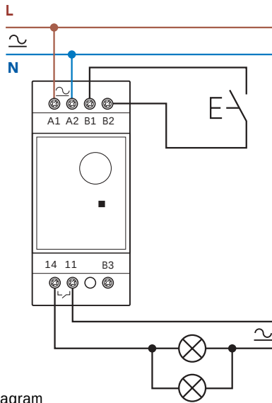
Type 13.01 Monostable wiring diagram
