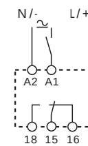
wiring diagram (without signal START)
