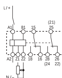
wiring diagram (without signal START)
