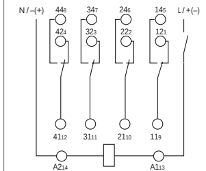
wiring diagram
