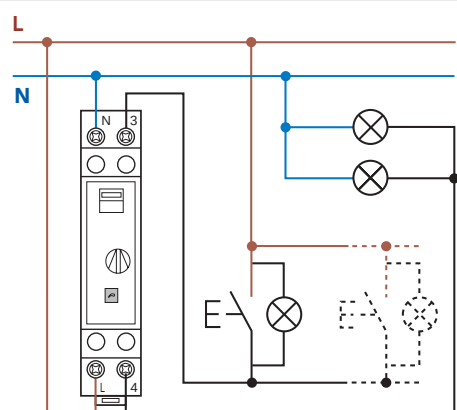
4 wire connection
