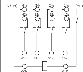
wiring diagram
