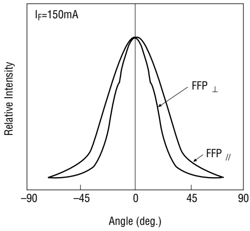
Far-Field Patterns
