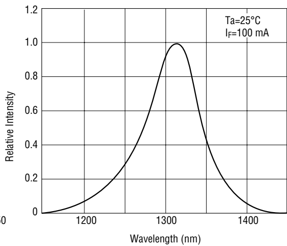
Emission Spectrum
