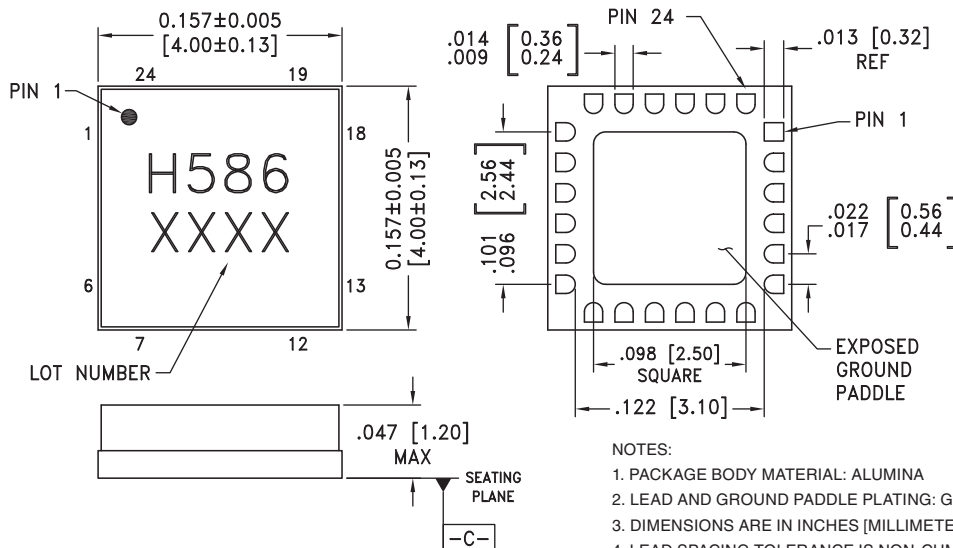
BOTTOM VIEW
