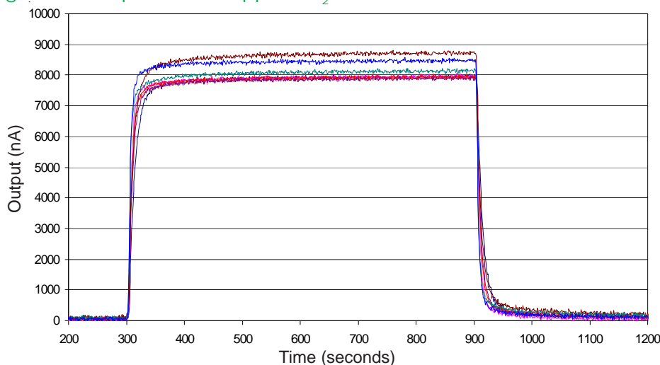
Figure 4 Response to 20ppm SO 2
