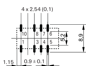
Short terminals
