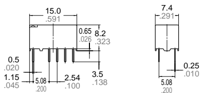
2 coil latching
