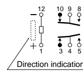
Single side stable (Deenergized condition)
