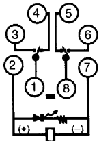
LED indicator type (DC coil) MK2PN-I, -S
