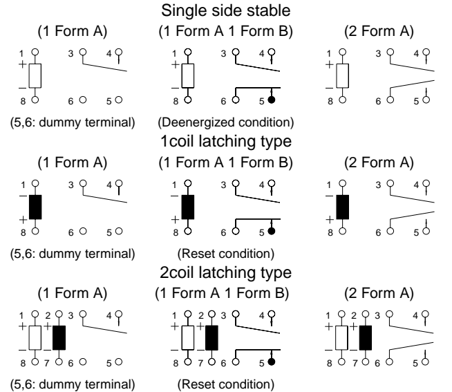
Schematic (Bottom view)
