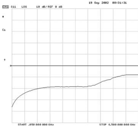
Return loss tested to 6.5 GHz for the CRF Reed Relay. Horizontal full scale: 6.5 GHz. Vertical scale: 10 dB/div referenced from the 0 mark.
