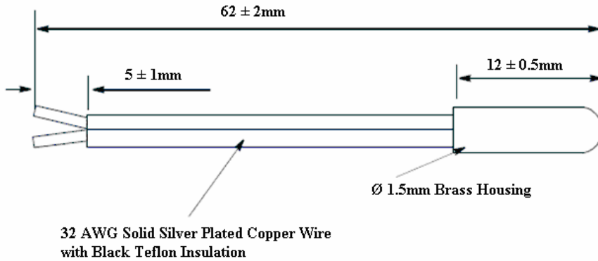
Figure 1: Fast time response probe
