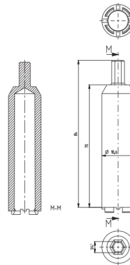
Screw insert
