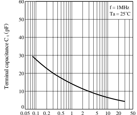
Fig. 6 Terminal Capacitance vs. Reverse Voltage
