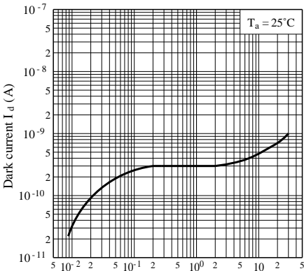
Fig. 5 Dark Current vs. Reverse Voltage
