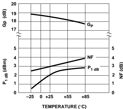
Figure 4. Output Power at 1 dB Gain Compression, NF and Power Gain vs. Temperature, f = 0.5 \text{ GHz} , I_d = 16 \text{ mA} .
