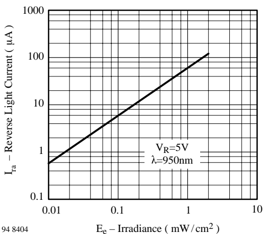
94 8404 E_e – Irradiance ( mW/cm^2 ) Figure 3. Reverse Light Current vs. Irradiance
