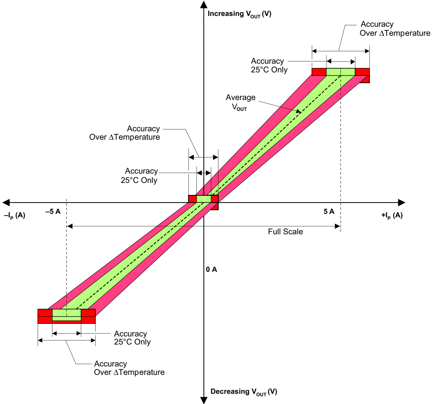
Output voltage vs. current, illustrating sensor accuracy at 0 A and at full-scale current
