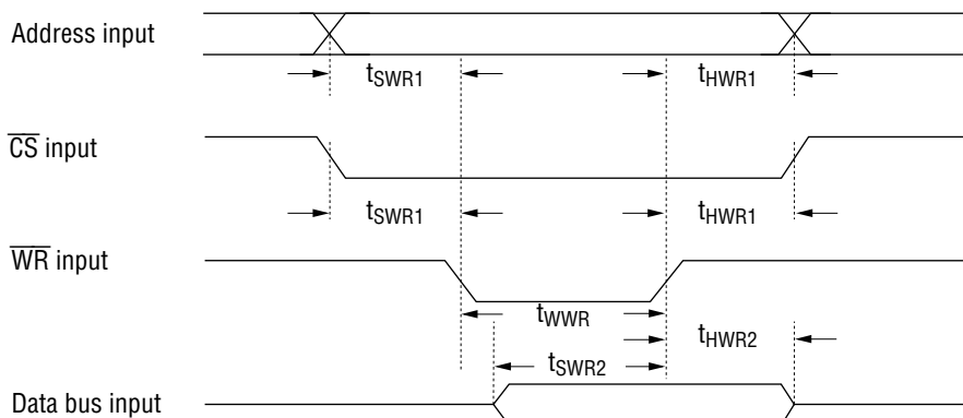
Figure 4.1 Write Timing
