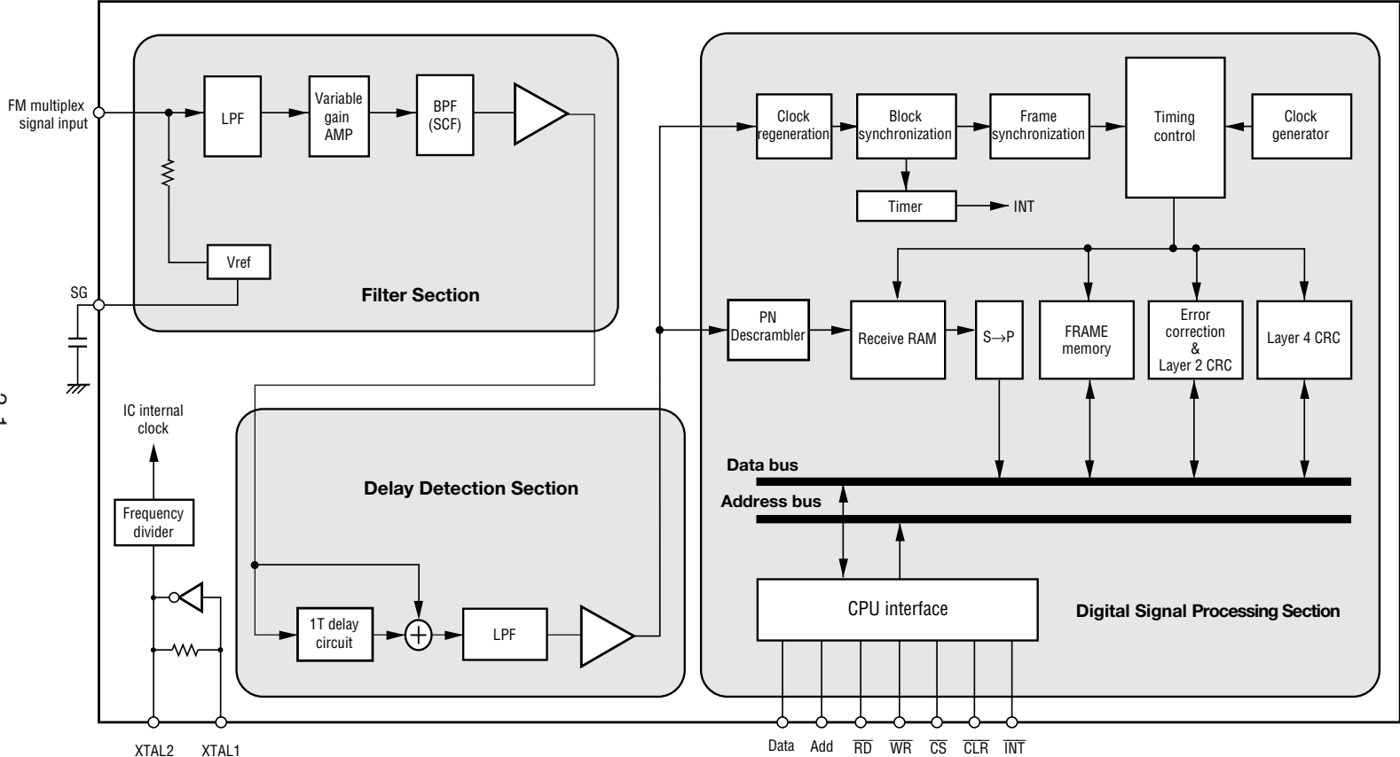
Figure 2.1 Block Diagram
