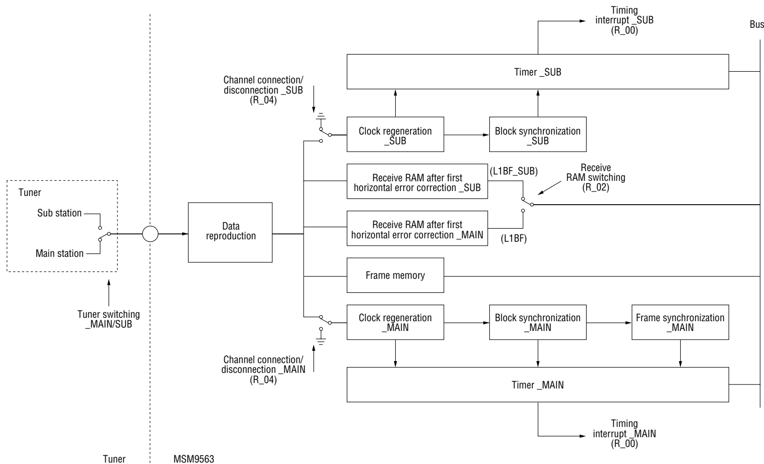
Figure 5.1 Main/Subchannel switching receive block diagram
