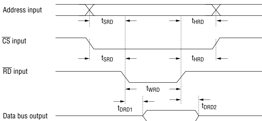
Figure 4.2 Read Timing
