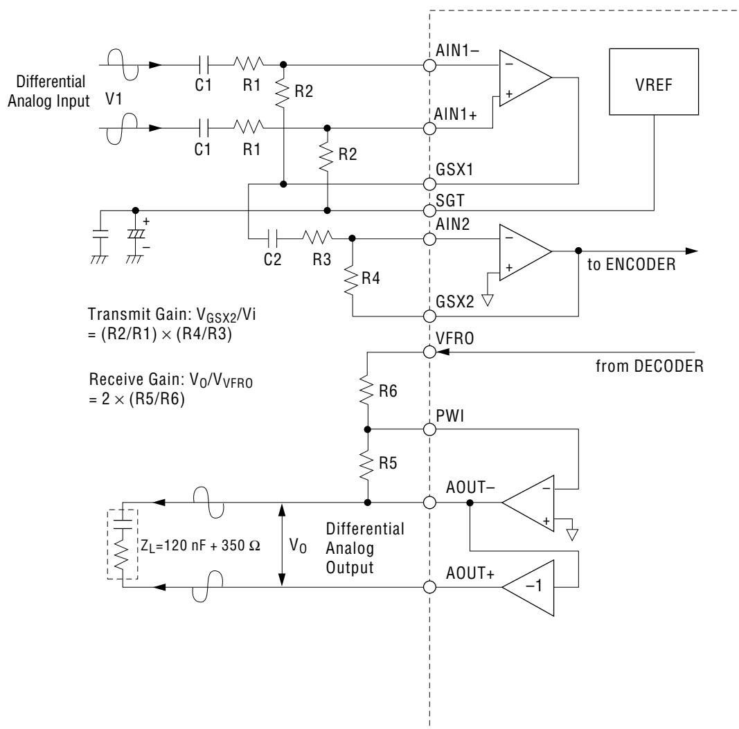
Figure 1 Analog Interface
