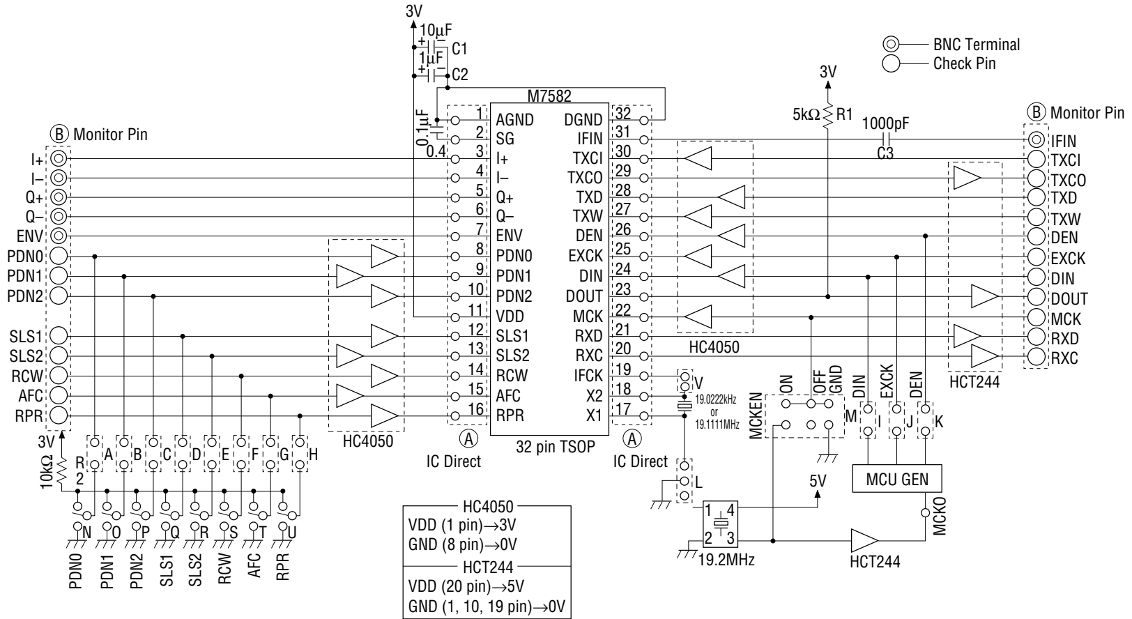
Fig. 1.1 MSM7582 Evaluation Board Circuit Diagram
