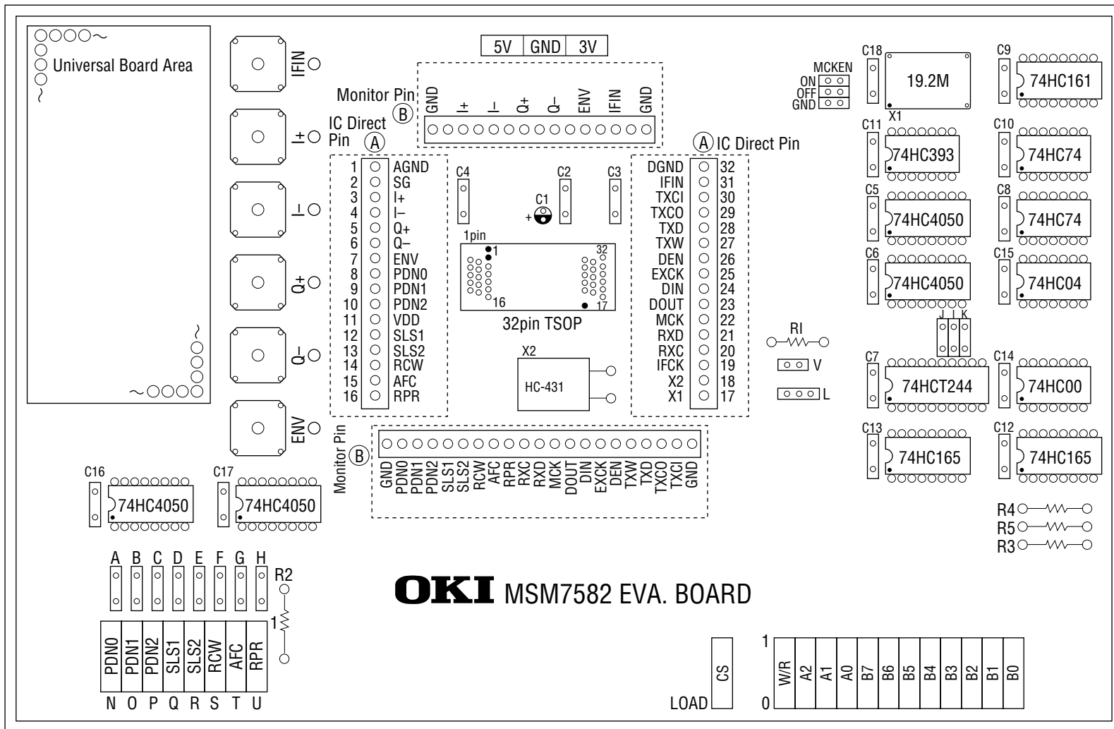
Fig. 2 MSM7582 Evaluation Board Layout
