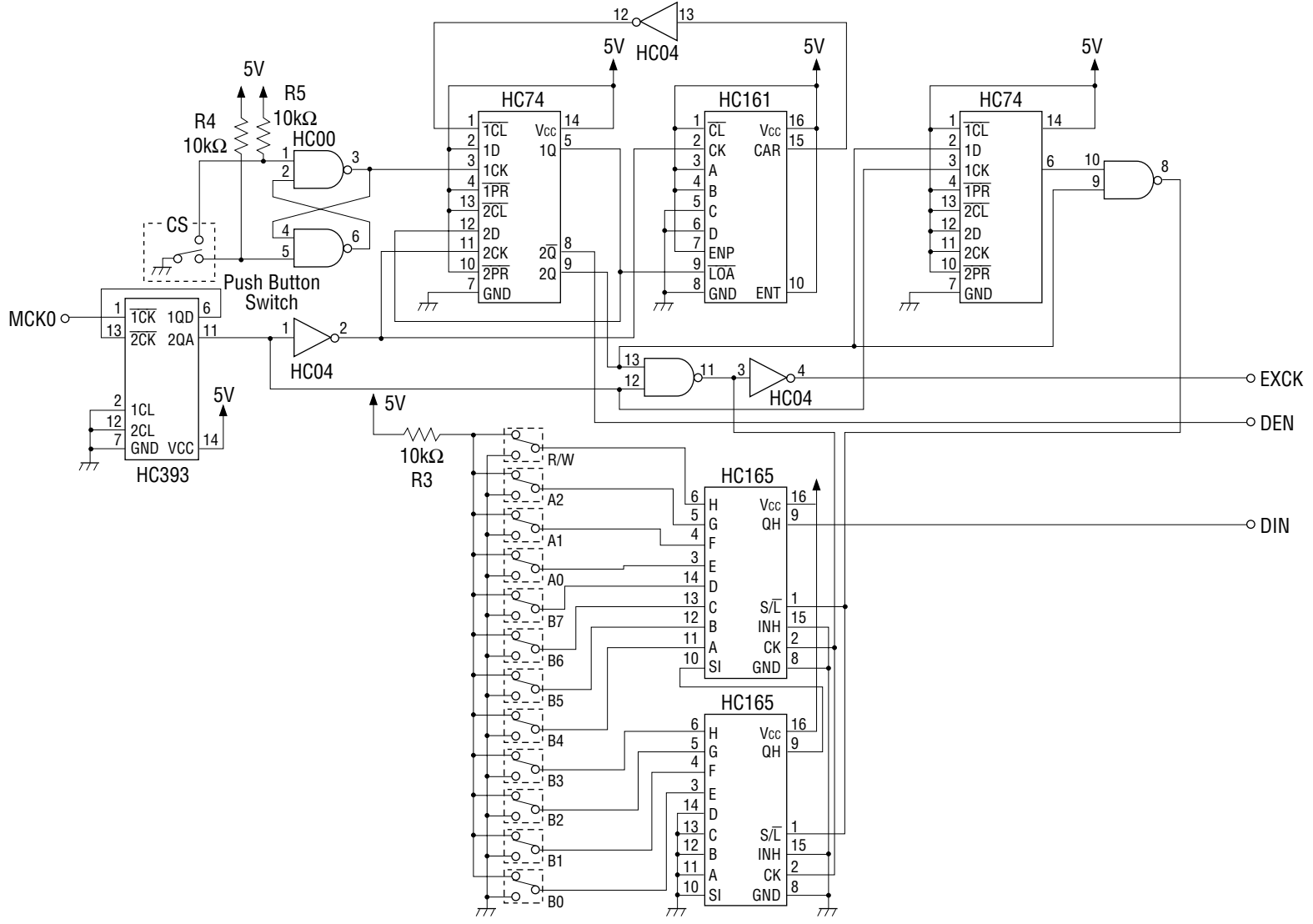
Fig. 1.2 MSM7582 Evaluation Board Circuit Diagram
