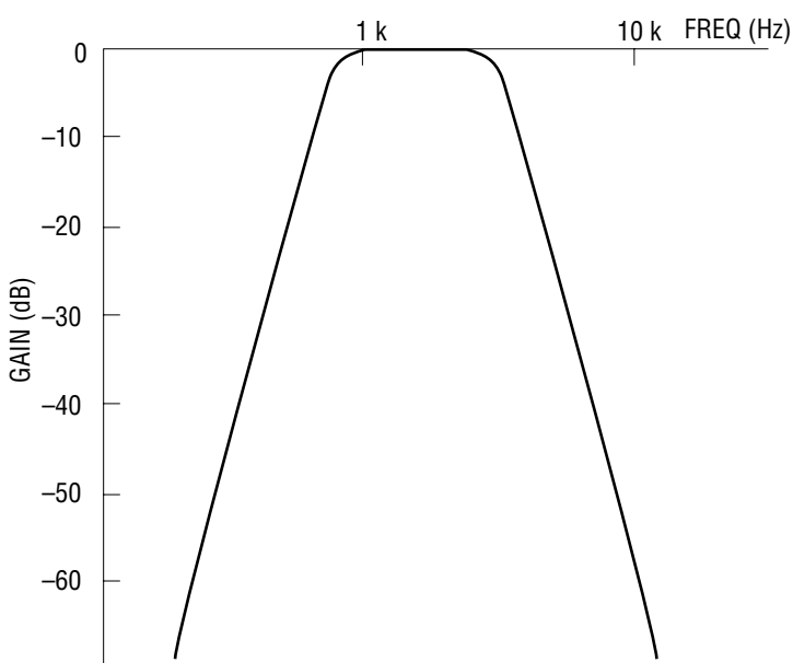
Figure 6 MSM6947 Receive Filter
