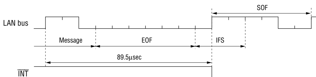
Figure 6-13 IFS Interrupt Generation Timing 1
