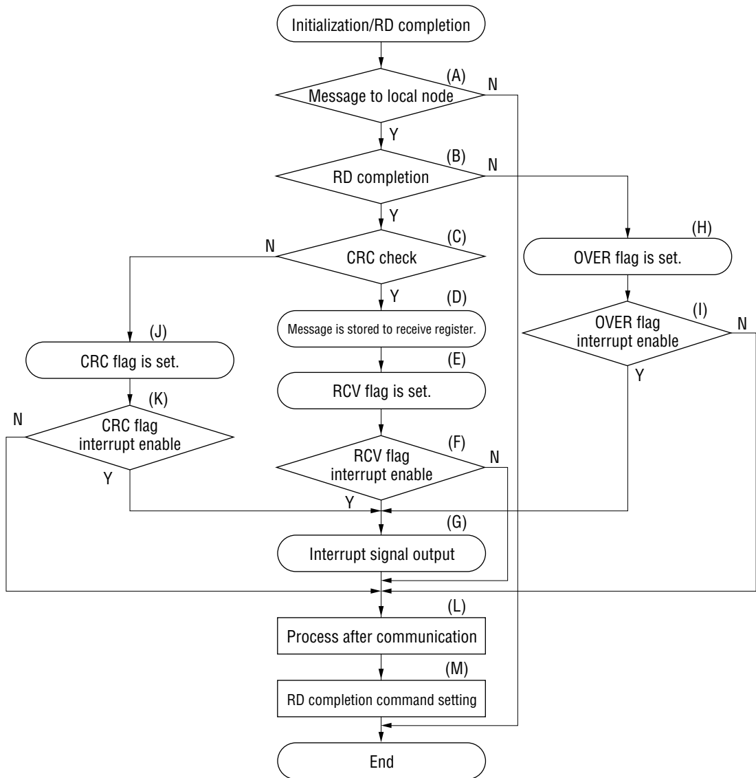
Figure 5-1 IFTR Type 0 Receive Flow
