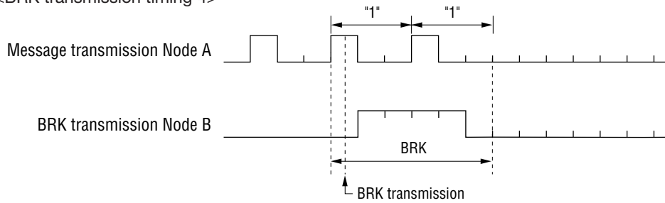
Figure 10-1 BRK Transmission Timing (2/2)
