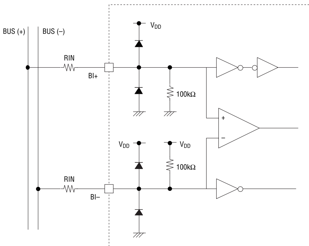
Figure 14-10 Internal Equivalent Circuit of LAN Bus Input Terminals BI+ and BI-
