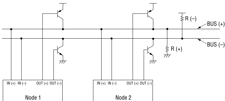
Figure 1-2 Configuration for J1850 LAN
