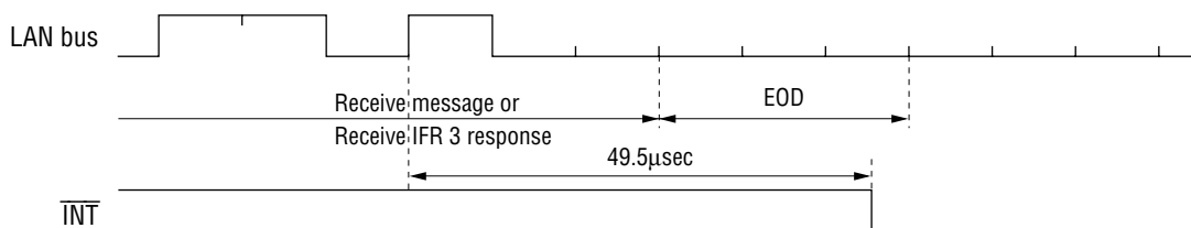
Figure 6-8 CRC Interrupt Generation Timing
