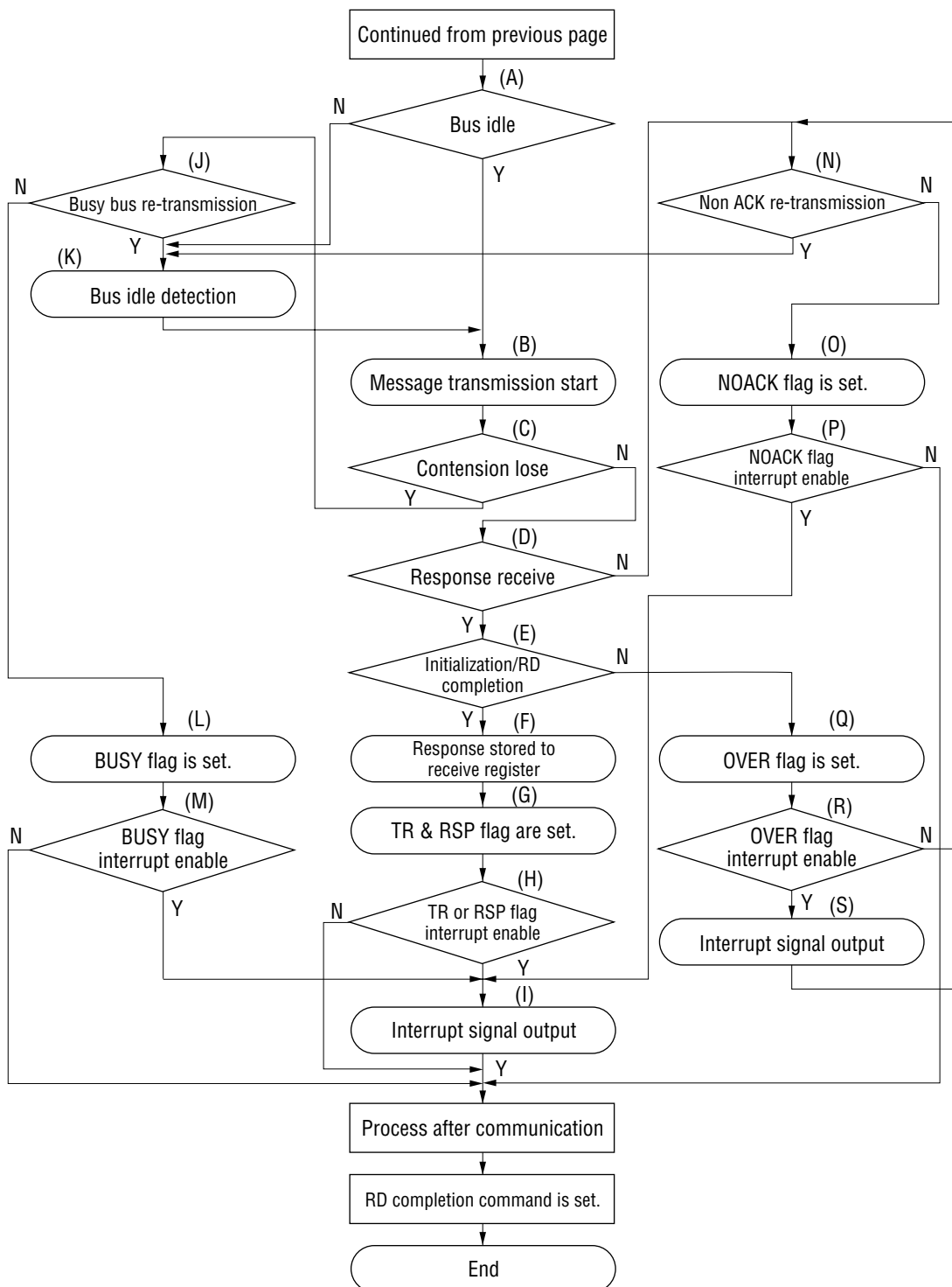
Figure 4-2 IFR Type 1 (1) Transmission Flow (2/2)
