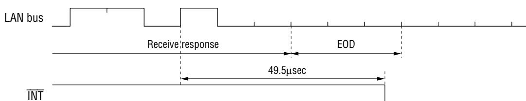
Figure 6-7 OVER Interrupt Generation Timing 2
