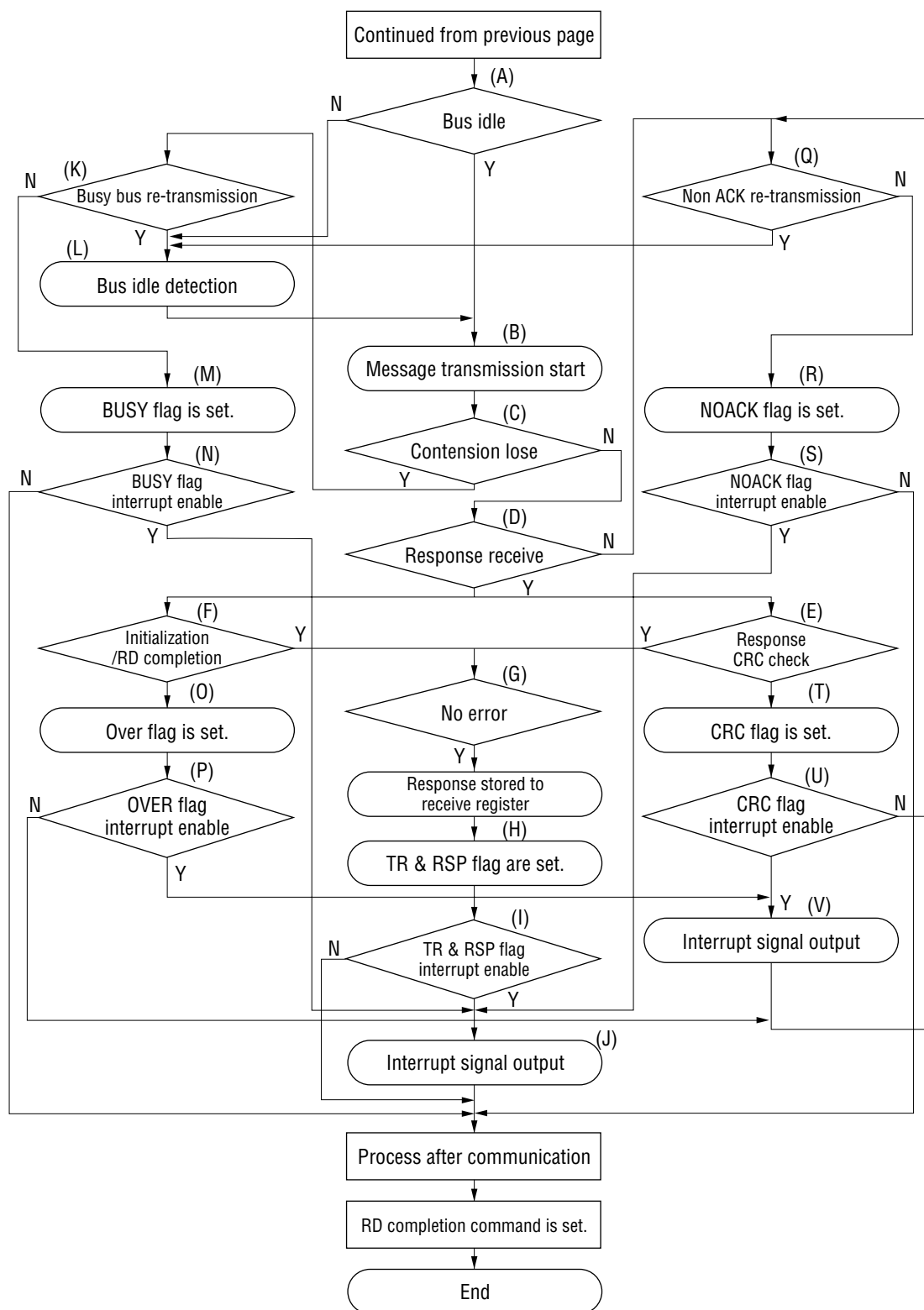
Figure 4-5 IFR Type 3 Transmission Flow (2/2)
