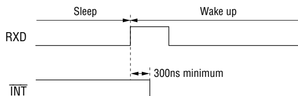
Figure 6-26 WAKR Interrupt Generation Timing
