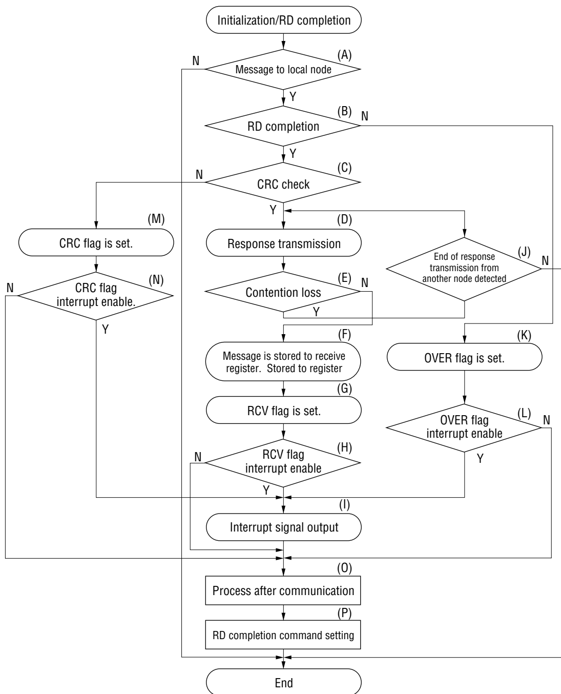
Figure 5-3 IFR Type 2 Receive Flow
