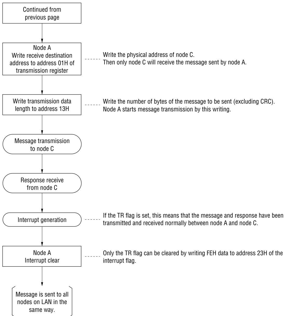
Figure 3-2 Network Initialization Flow (2/2)
