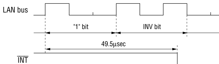
Figure 6-12 INV Interrupt Generation Timing
