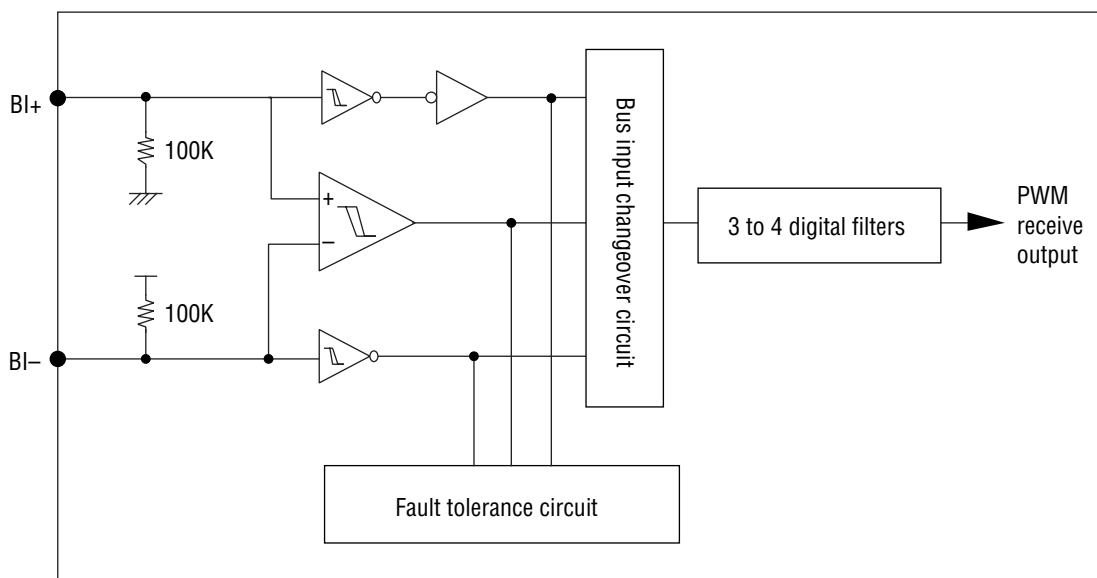
Figure 12-1 Bus Receiver
