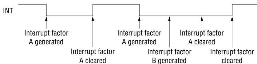
Figure 6-1 Clearing Interrupt Request
