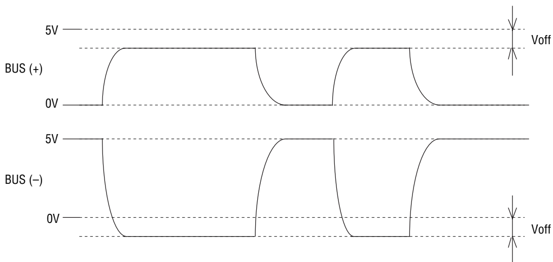
Figure 14-9 LAN Bus Waveforms with GND Offset
