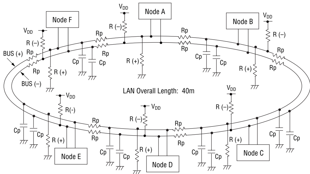
Figure 14-5 LAN Configuration Example 3
