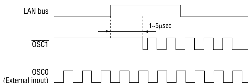
Figure 8-3 LAN Bus Wake Up
