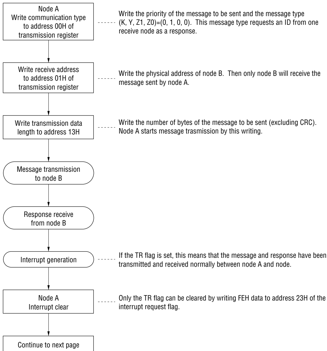
Figure 3-2 Network Initialization Flow (1/2)
