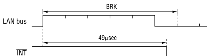
Figure 6-20 BRK Interrupt Generation Timing
