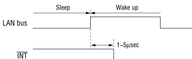
Figure 6-27 WAKD Interrupt Generation Timing
