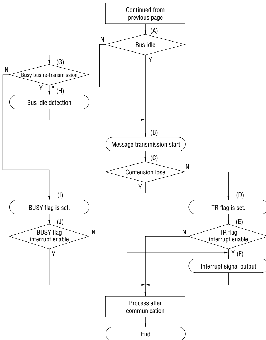
Figure 4-1 IFR Type 0 Transmission Flow (2/2)
