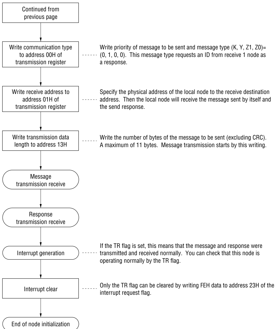
Figure 3-1 Node Initialization Flow (2/2)
