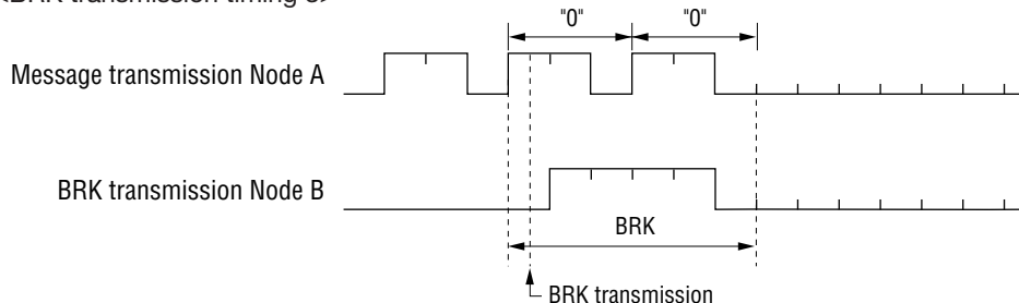
Figure 10-1 BRK Transmission Timing (1/2)
