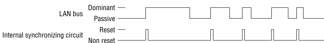
Figure 1-5 Synchronization of J1850
