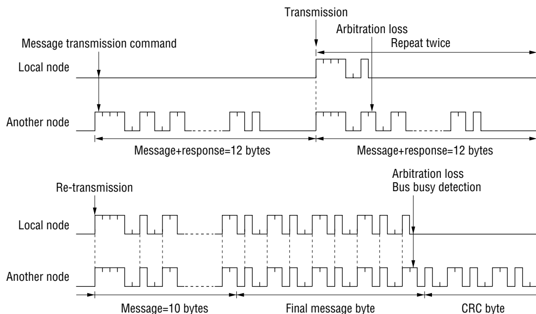
Figure 6-16 Maximum BUSY Interrupt Generation Time
