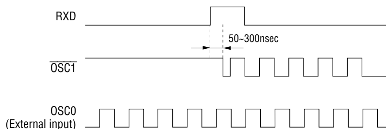
Figure 8-4 RXD Wake Up
