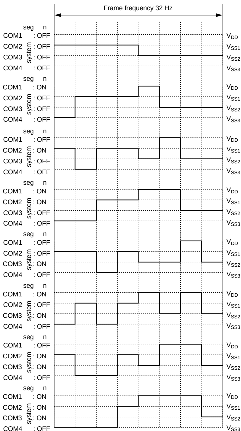
Figure 13-6 (b) 1/4 Duty Common Driving Waveforms (1/3 bias)
