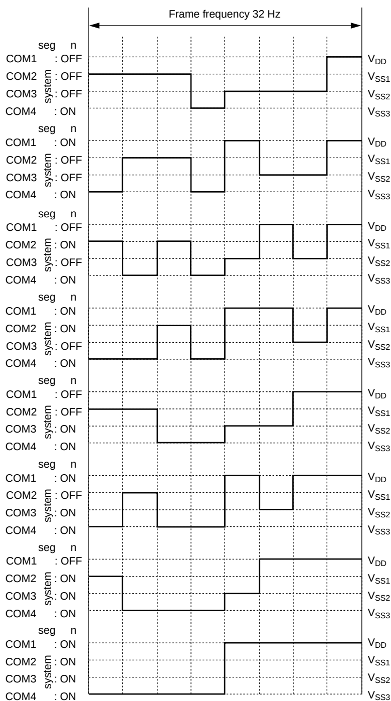
Figure 13-6 (c) 1/4 Duty Common Driving Waveforms (1/3 bias)
