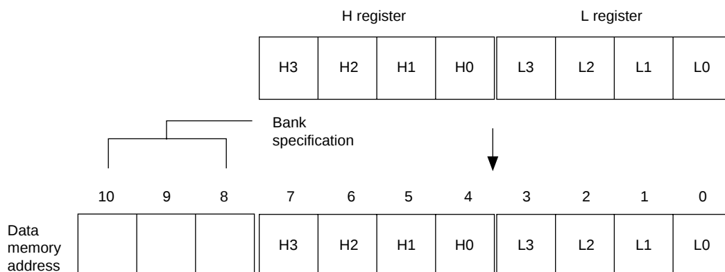
Figure 2-7 Data Memory Address of HL Indirect Addressing
