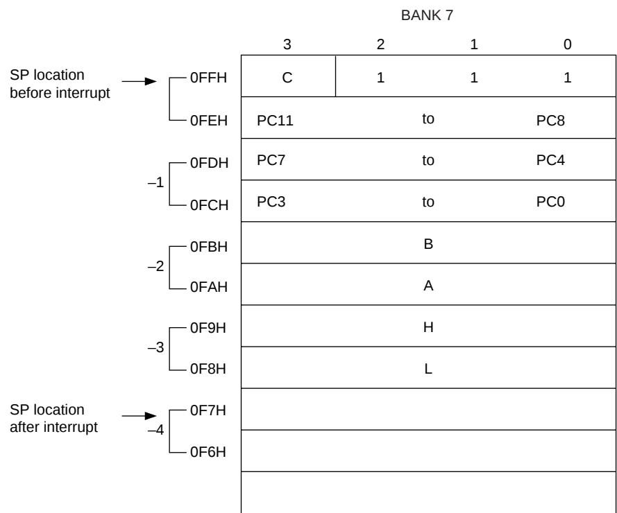
Figure 4-2 Contents of Stack after Interrupt Generation
