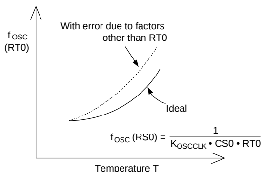
Figure 12-12 Oscillation Characteristics of Thermistor
