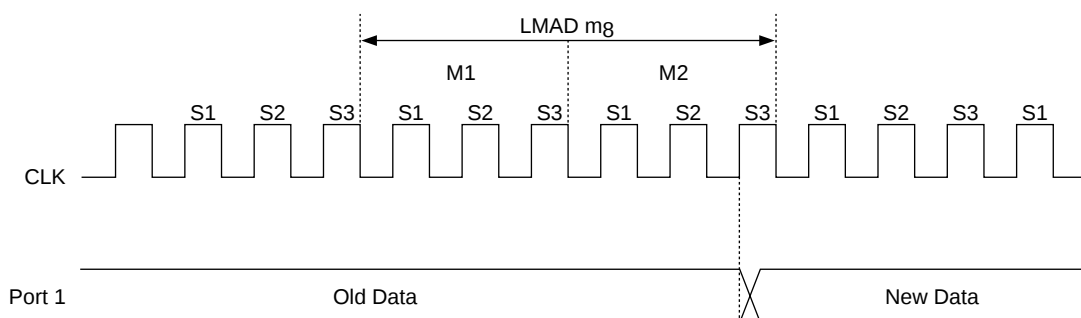
Figure 7-3 Example of Writing to Port Data Register by "LMAD mg" Instruction
