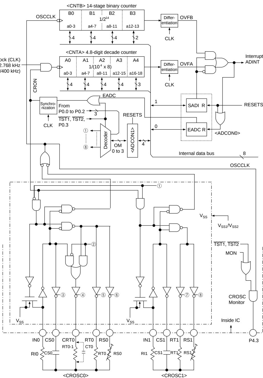
Figure 12-1 Layout of A/D Converter
