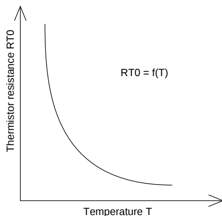
Figure 12-9 Temperature Characteristics of Thermistor
