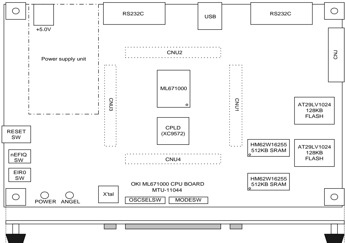
Figure 3. ML671000 CPU Board Layout
